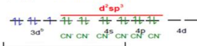
Figure 35 Type of Hybridization in ligand environment
