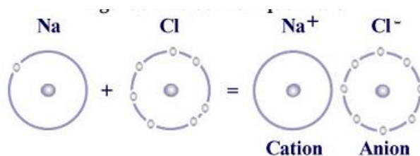
Figure 2 Ion bonding
