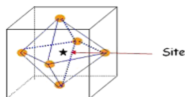
Figure 12 Octahedral sites
