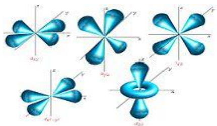
Figure 36 : Representation of the Five d Orbitals
