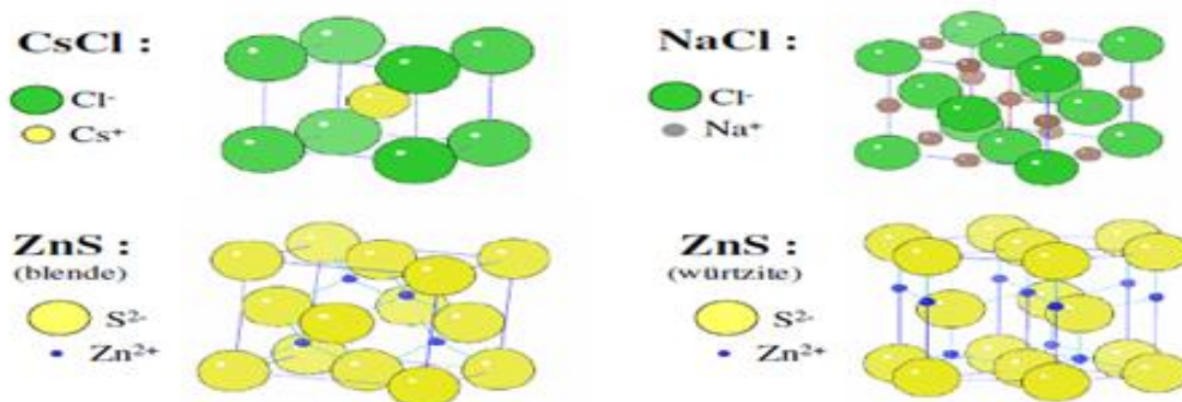
Figure 17 : MX type structures
