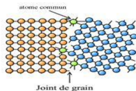
Figure 9: Grain boundaries
